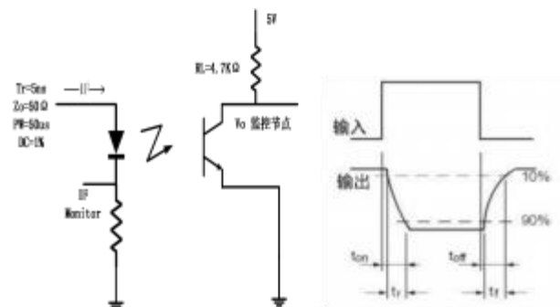
Fig.11 Switching Time Test Circuit & Wave forms
