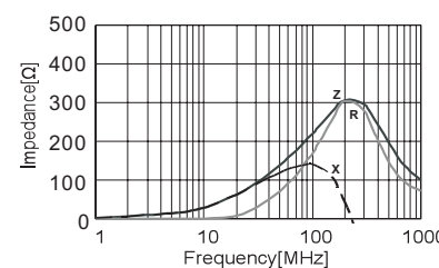
CBW321609U221T
