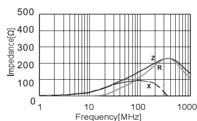
CBW321609U151T
