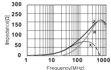
CBW100505U101T
