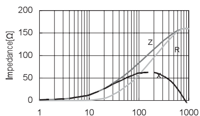
CBW201209U800T
