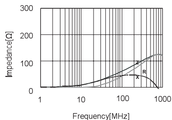
CBW322513U600T
