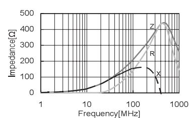
CBW100505U201T
