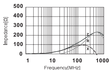
CBW100505U121T
