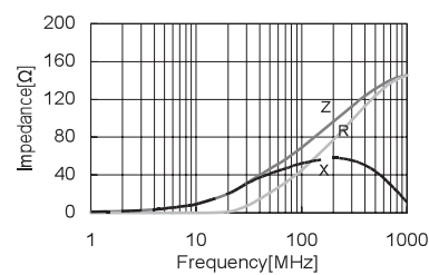
CBW453215U700T
