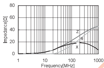
CBW322513U190T
