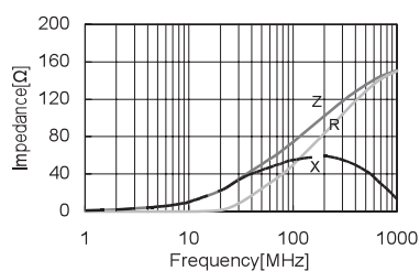
CBW453215U800T
