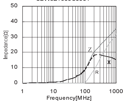
CBW321609U090T
