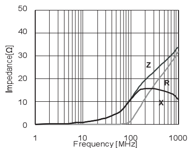
CBW160808U110T
