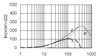
CBW201209U151T
