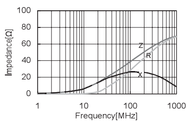
CBW453215U380T
