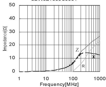
CBW321609U050T
