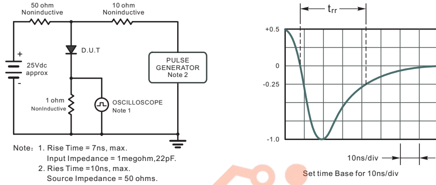
Fig.3 Typical Reverse Characteristics
